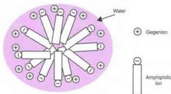
Spherical micelle of an anionic association colloid in aqueous media
